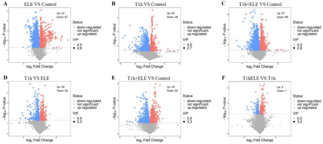
Figure S2. The Volcano plot of muscle metabolites in pairwise comparison. Metabolites in red were up-regulated and metabolites in blue were down-regulated. Differential metabolites marked in the plot were determined by combining restrictions of p < 0.05 and VIP > 1.0 .
