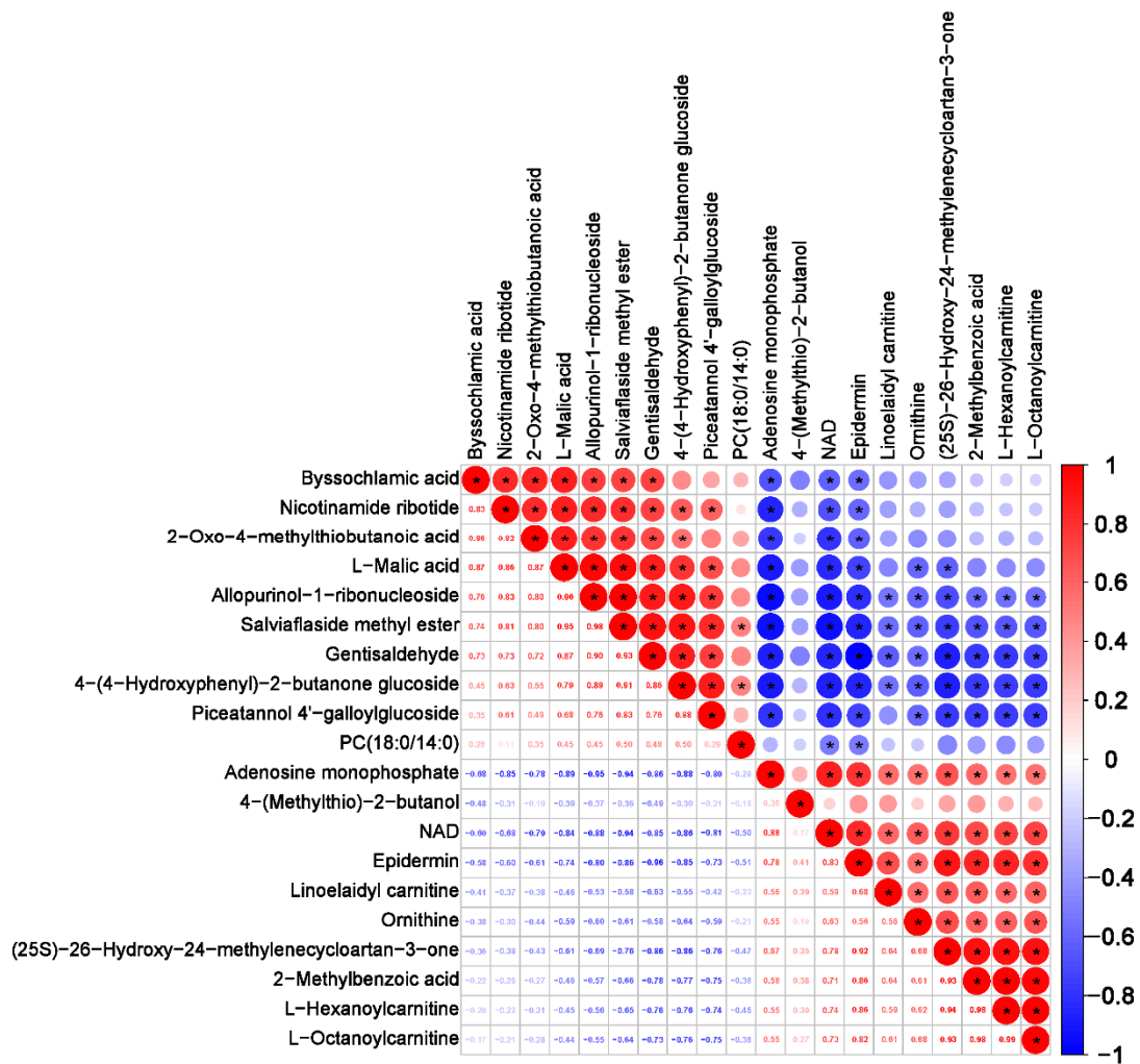
Figure S2. Correlation analysis of different metabolites in goat sperm between control group and sodium salicylate (SS) group. * means significant. r is the correlation coefficient, and the closer the absolute value of r is to 1, the stronger the correlation between the two variables.
